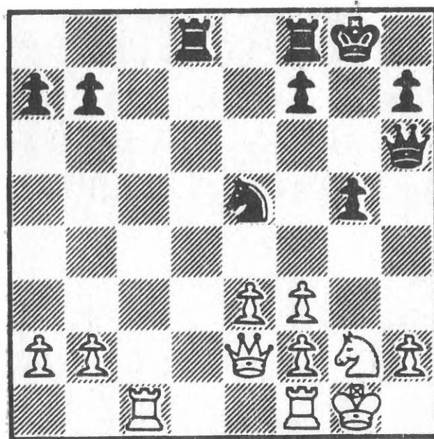
500 After 20 Ng2
